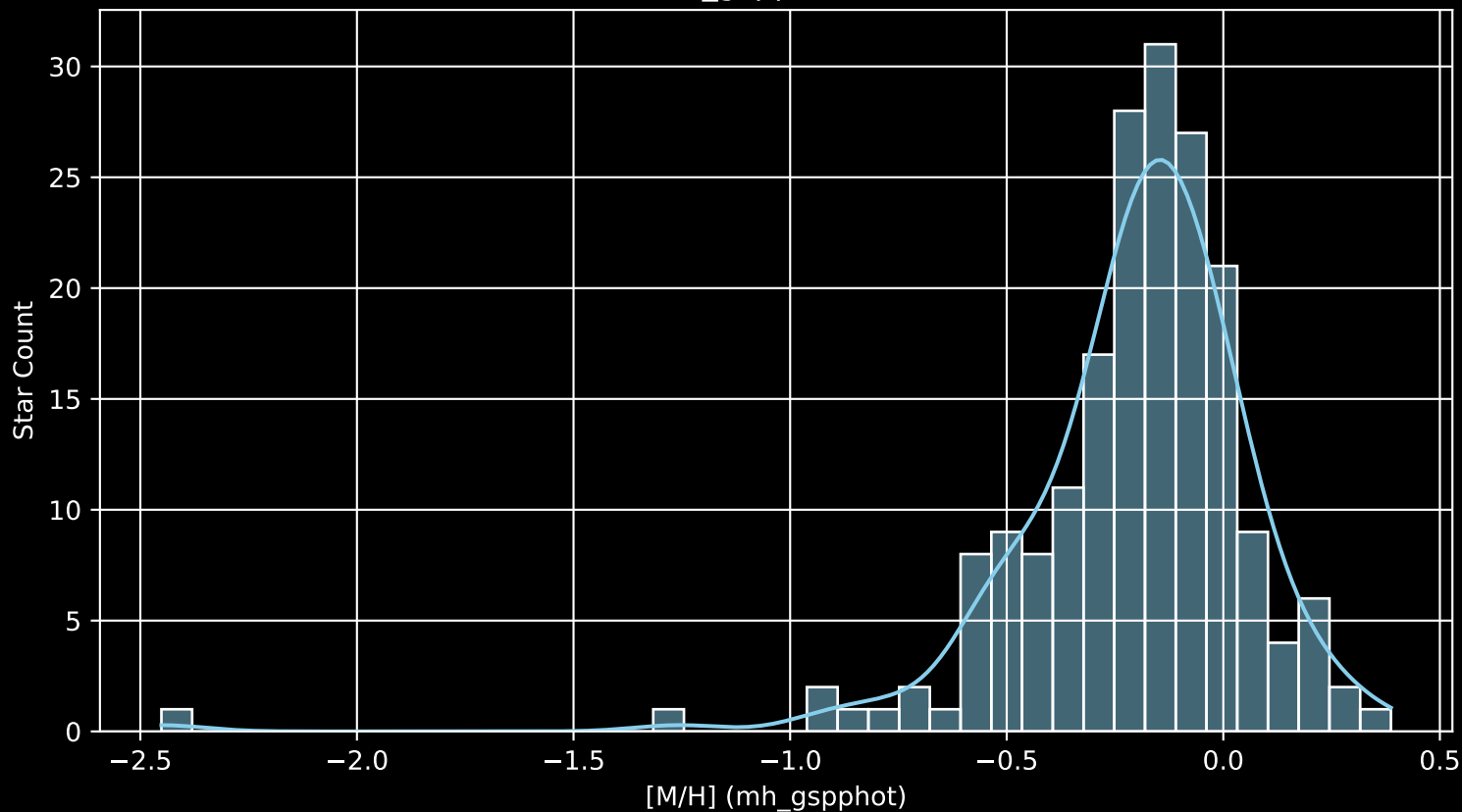
APOGEE DR17 Field: [NGC2420_bt [M/H] (mh_gspphot) (n= 191)
