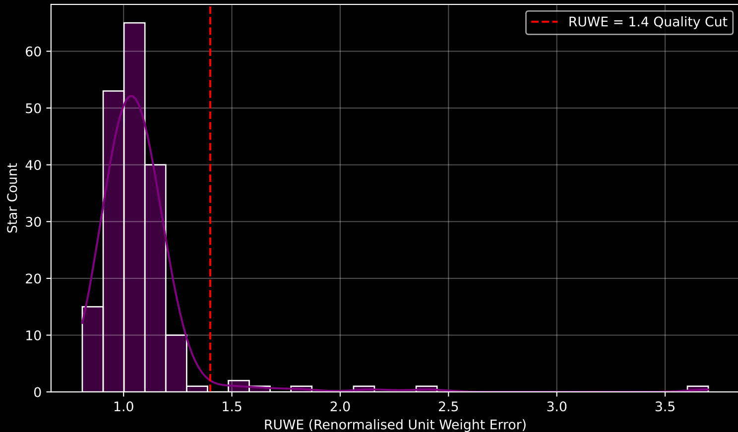
GAPOGEE DR17 Field [NGC2420_btx] RUWE Distribution (n= 191)
