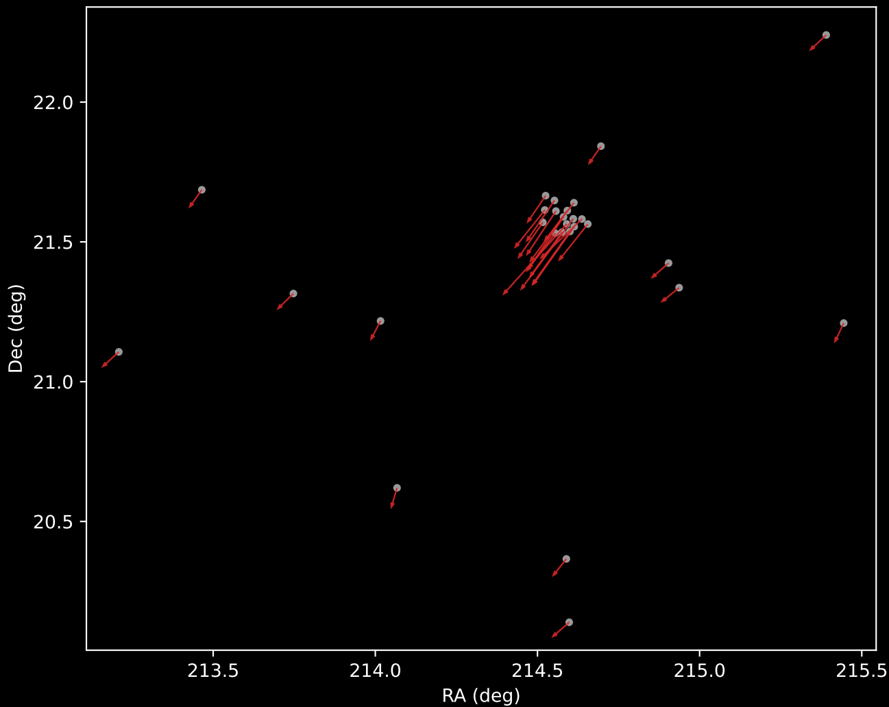
APOGEE DR17 Cluster 6 Proper Motion Vectors (n=28)
