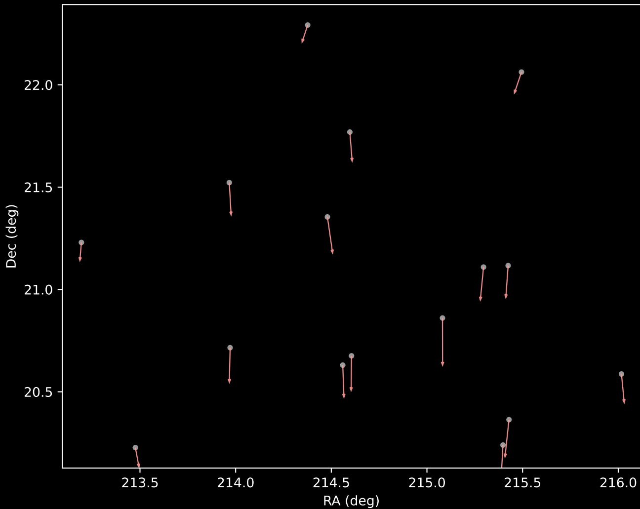
APOGEE DR17 Cluster 7 Proper Motion Vectors (n=16)
