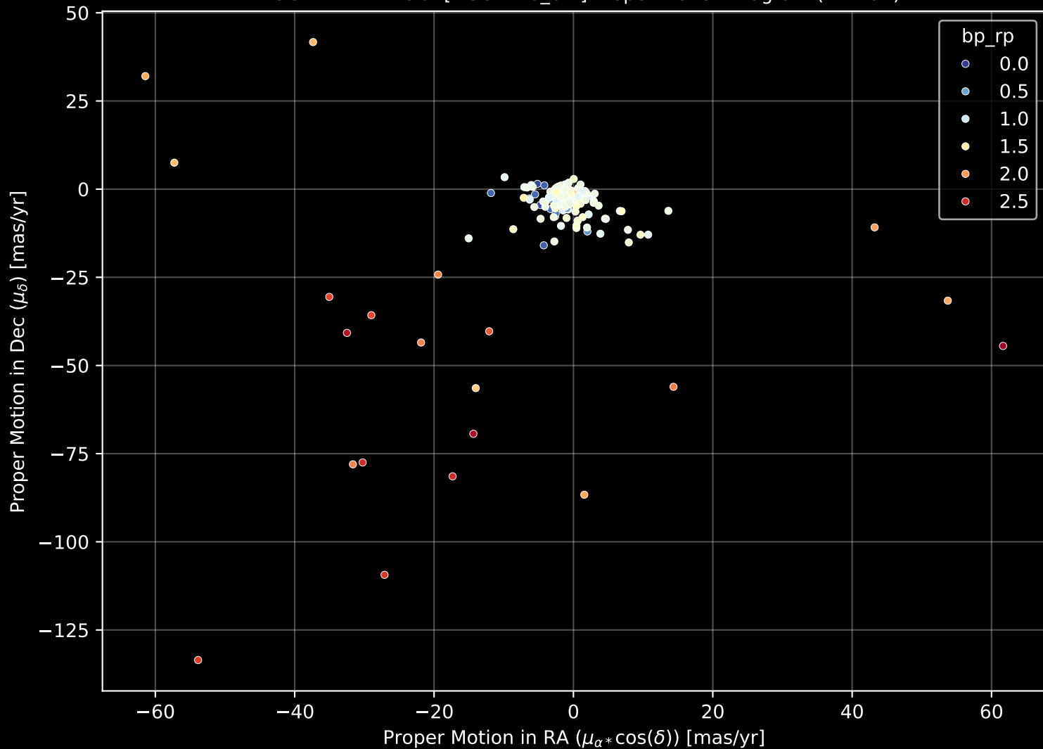
APOGEE DR17 Field: [NGC2420_btx] Proper Motion Diagram (n= 192)
