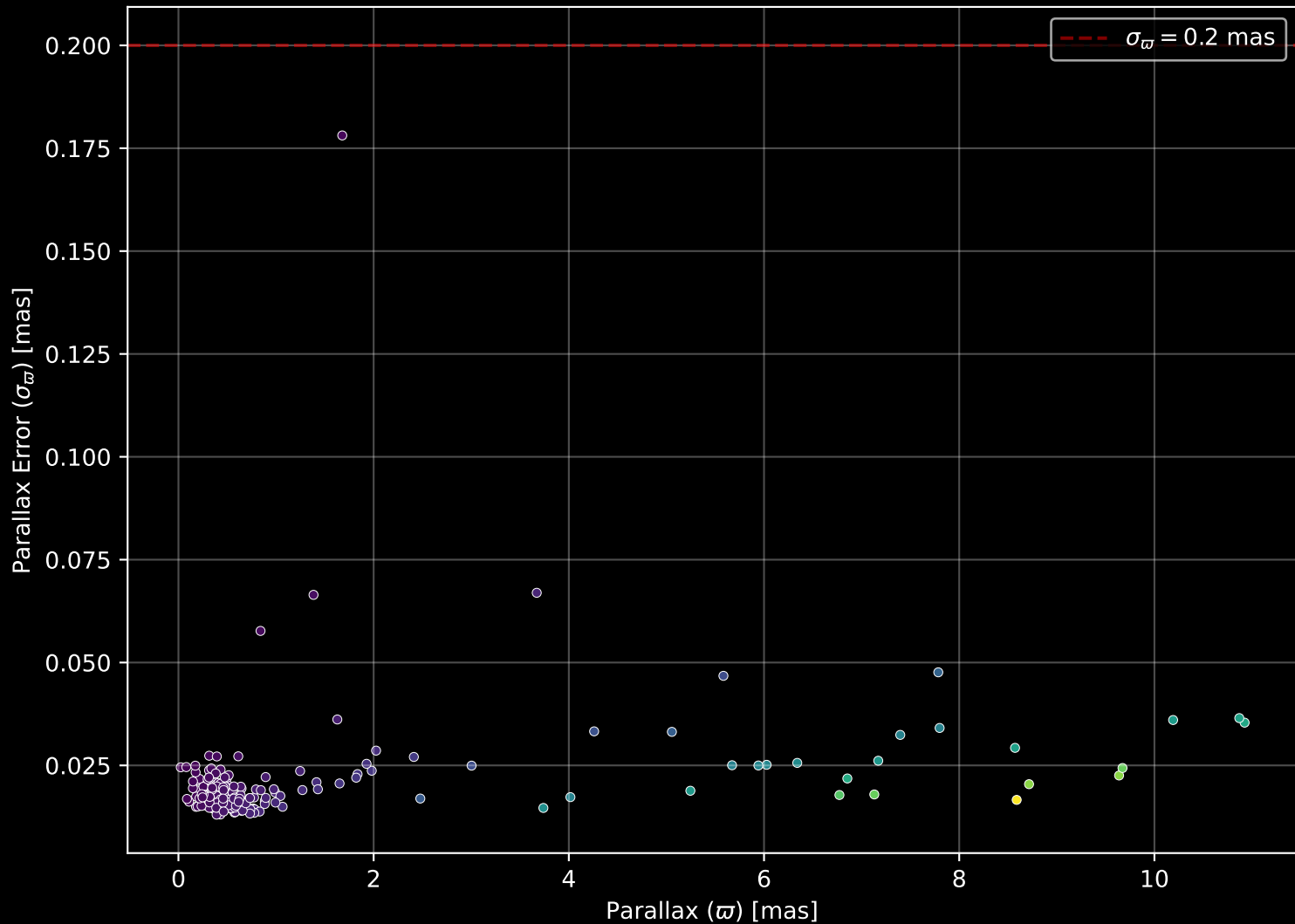
APOGEE DR17 Field: [NGC2420_btx] Parallax Quality (n= 192)
