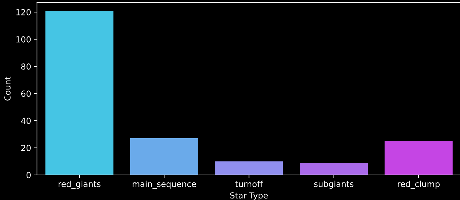
APOGEE DR17 Field: [NGC2420_btx] Count plot of Star Type
